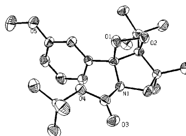
Figure 1. ORTEP view of dioxetane 2a .
